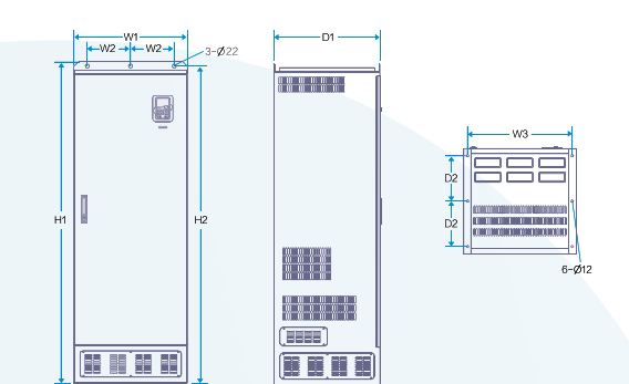
355-500kW Floor mounting Installation diagram
