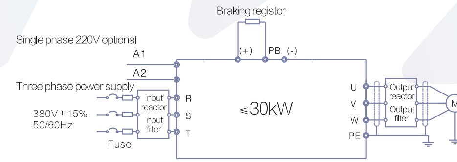
Wiring diagram of the main circuit
